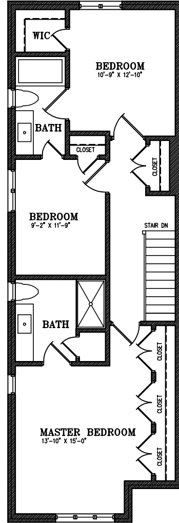
SECOND FLOOR PLAN 910 SF
