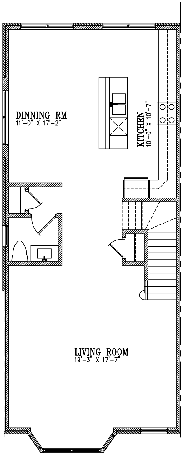
FIRST FLOOR PLAN UNIT E
