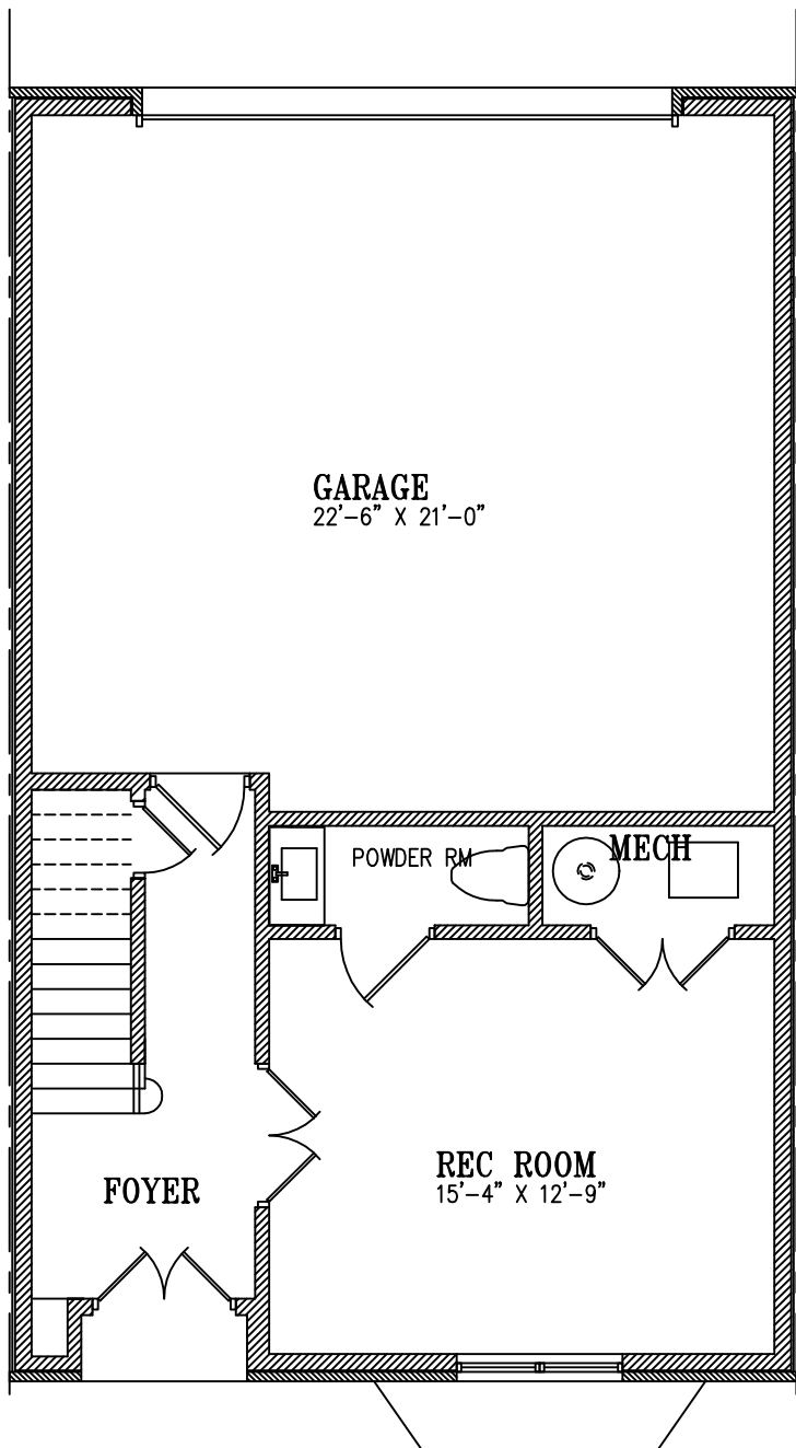
FLOOR PLAN LOWER LEVEL UNIT E
